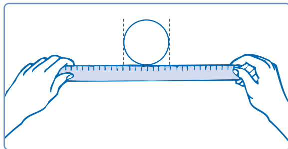
▲ Figure 5-2. Measuring Earth's diameter.
