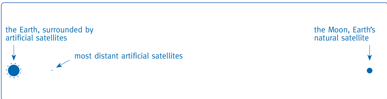
▲ Figure 5-3. An accurate distance model of Earth and its satellites (not accurate to size).
