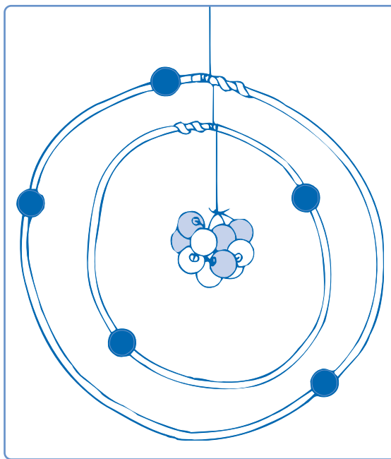
▲ Figure 4-2. A model boron atom.
